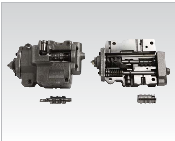
HYDRAULIC PUMP COMPONENTS (REGULATOR assembly)
